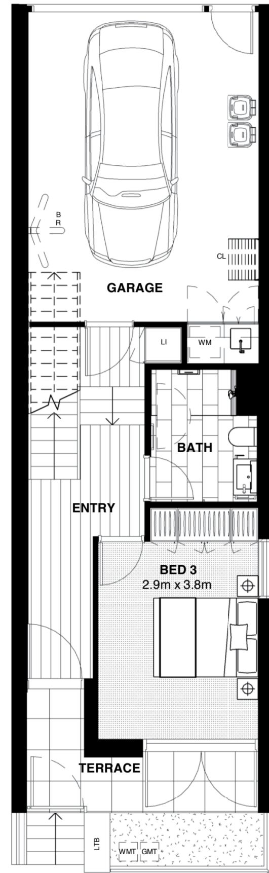
GROUND FLOOR
